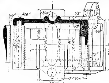
Fig. 5140. Sectional Plan.
